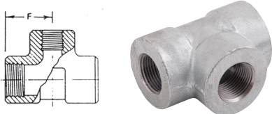
Female Thread, NPT
