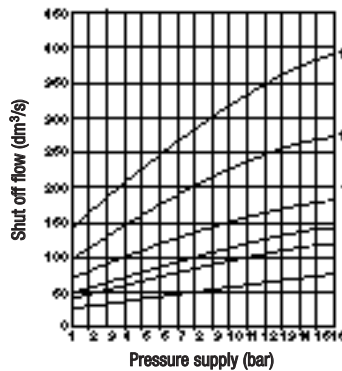
Flow (±10%) vs pressure supply (3/4 ... 1½")
