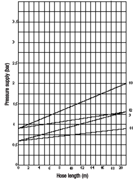
Hose length vs minimum pressure supply (1" ... 1½")
