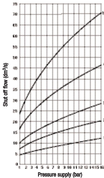
Flow (±10%) vs pressure supply (1/4 ... 1/2")
